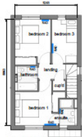
first floor, type 3BF & 3BFH plot 2,3,4,6,7,8,10,11,12
