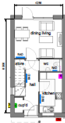
ground floor 1:100
